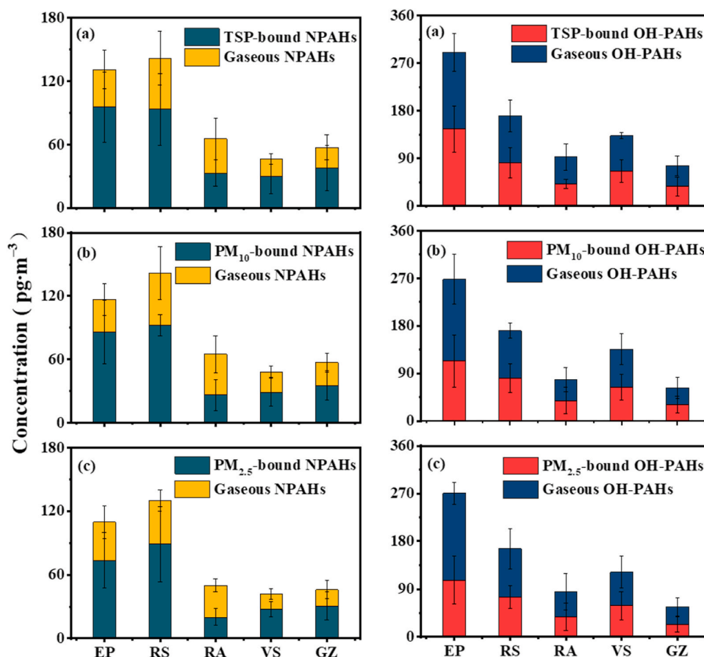
Fig. 2. Concentrations of NPAHs and OH-PAHs in particulate (TSP, PM 10 , and PM 2.5 ) and in gaseous phases at different sampling sites.
