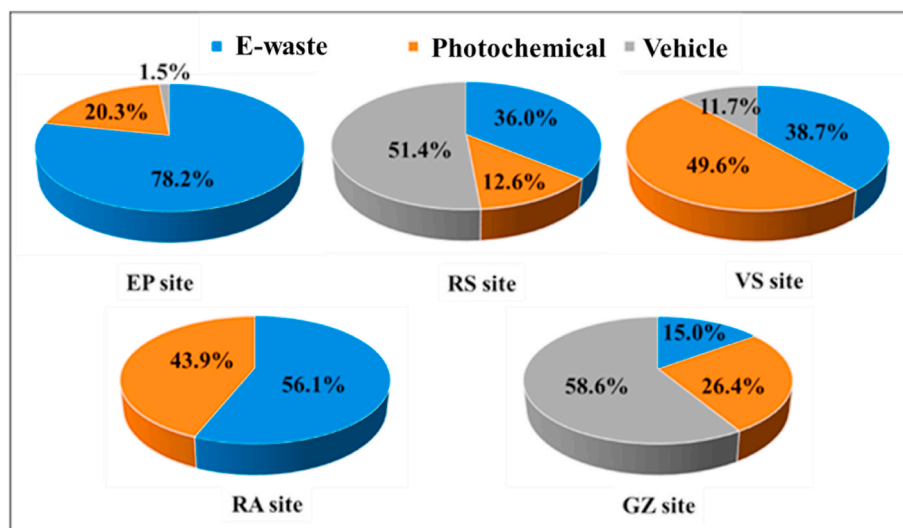
Fig. 5. Source contributions (%) of NPAHs at different sampling sites.
