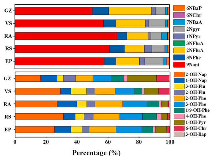
Fig. 3. Composition profiles of NPAH (a) and OH-PAHs (b) in the atmospheric samples collected at different sampling sites.
