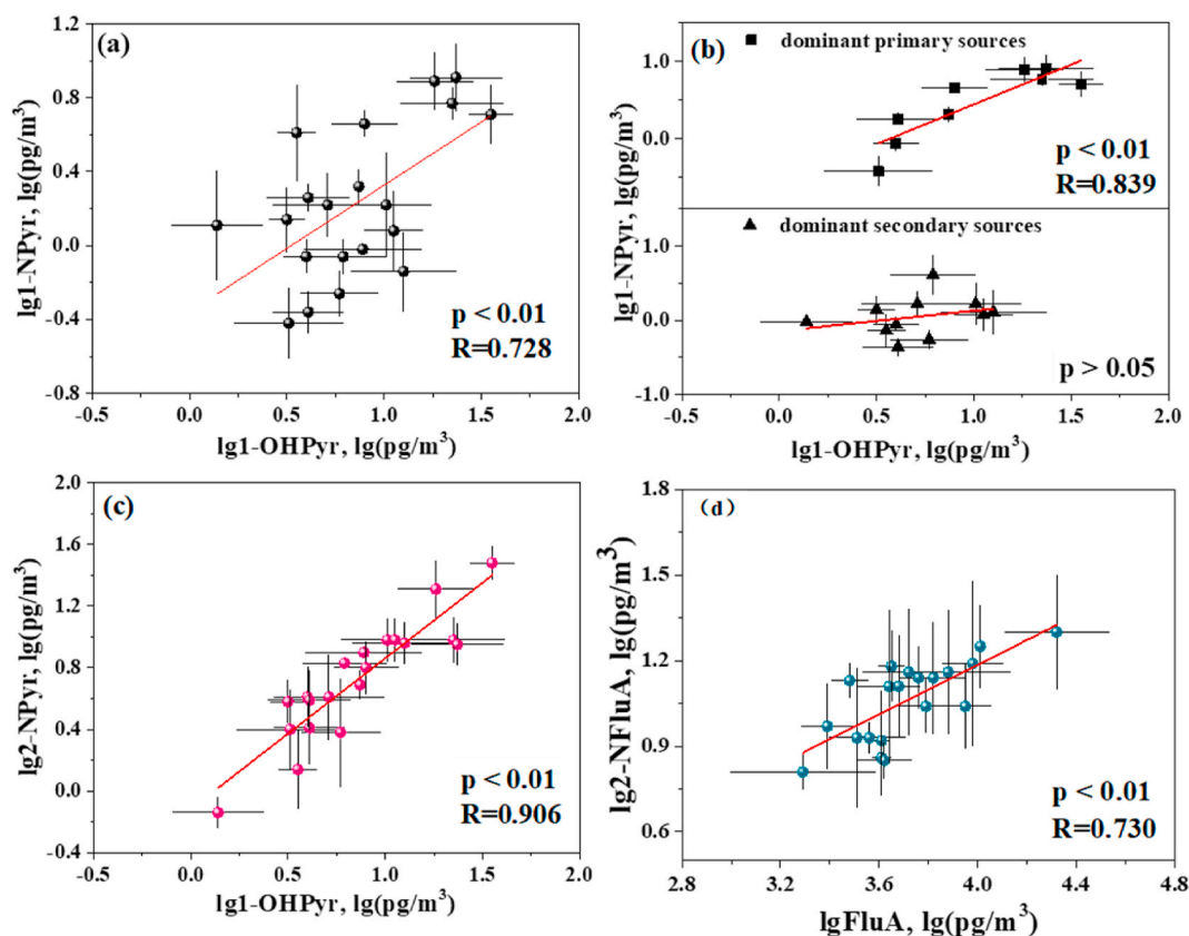
Fig. 6. Correlations between 1-OHPyr and 1-NPyr (a: total; b: predominantly primary or secondary sources, respectively), 1-OHPyr and 2-NPyr (c), and 2-NFluA and FluA (d) at the e-waste dismantling area.
