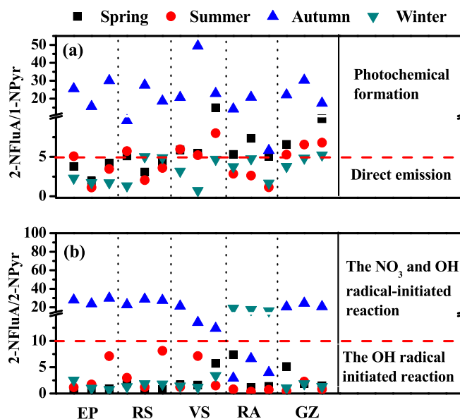
Fig. 4. The concentration ratios of 2-NFluA/1-NPyr (a) and 2-NFluA/2-NPyr (b) at different sampling sites.
