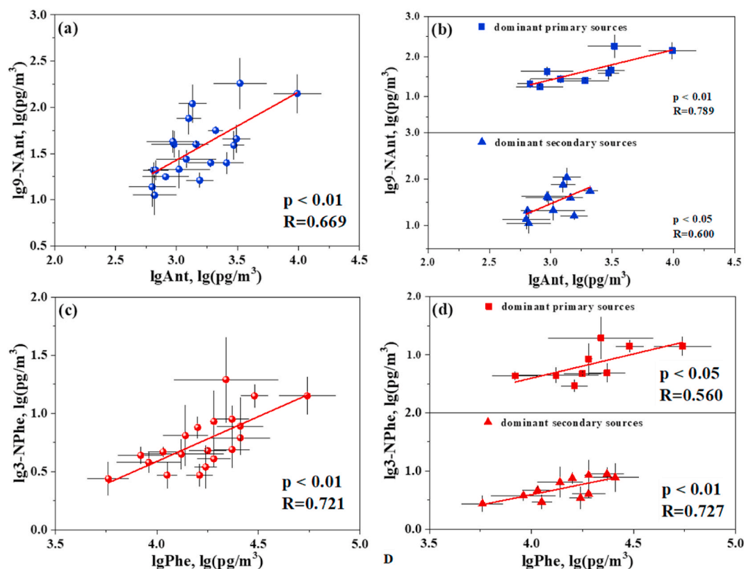
Fig. 7. Correlations between 9-NAnt and Ant, 3-NPhe and Phe (a or c: total; b or d: predominantly primary or secondary sources, respectively) at the e-waste dismantling area.
